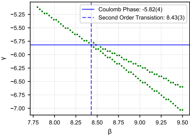
A5 Phase Diagram for Adjoint rep 3^{(0)}
